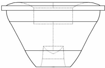
图 2 小角度透镜的二维轮廓 Fig. 2 Two-dimensional profile of small angle lens
